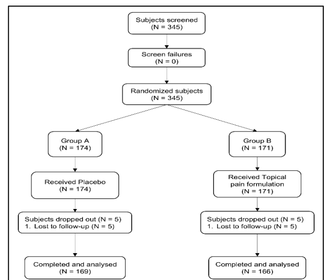
Figure 1: Participants flow.
